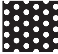
3/32" @ 3/16" STAGGERED Open area . . . 23%
