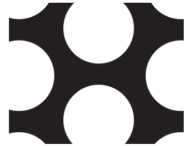
1/2" @ 11/16" STAGGERED Open area . . . 47%
