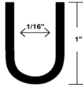
18 GA #403 U-EDGING
