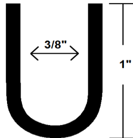
18 GA #438 U-EDGING
