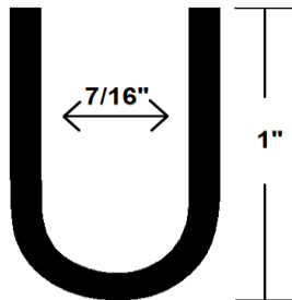
18 GA #437 U-EDGING
