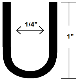
18 GA #401 U-EDGING
